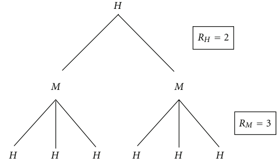
FIGURE 1: A example of a two-stage basic reproductive ratio. A single human infects R_H = 2 mosquitoes, each of whom subsequently infects R_M = 3 humans. Thus, a single human results in R_0 = 6 infected humans. The next-generation method instead estimates R_{0,N} = \sqrt{6} infected individuals in the subsequent generation, regardless of whether that generation is human or mosquito; R_{0,N} is the geometric mean of R_H = 2 and R_M = 3 . (Reproduced with permission from Smith? [7]).
